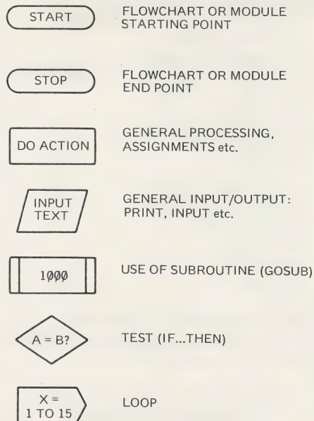
Fig 3. Some typical flowcharting symbols.
